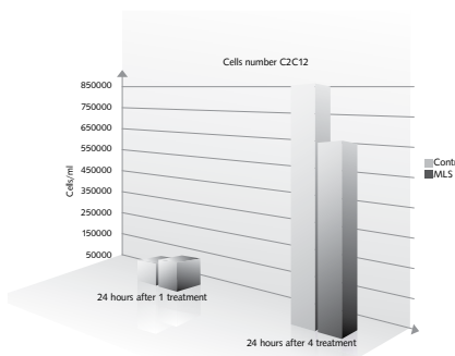
Fig. 2. C2C12 Cell proliferation assessed 24 h after 1st MLS treatment and 24 h after the fourth MLS treatment. (Control vs. MLS). Data were obtained by Trypan Blue assay.
