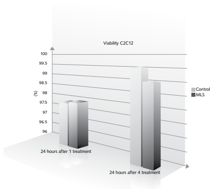
Fig. 1. C2C12 Cell viability assessed 24 h after 1st MLS treatment and 24 h after the fourth MLS treatments. (Control vs. MLS). Data were obtained by Trypan Blue assay.
